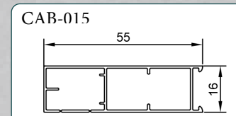
CAB-015 FRONT PANEL BOARD
