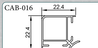
CAB-016 CORNER CONNECTOR
