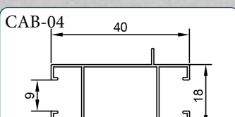
CAB-04 DIVIDER
