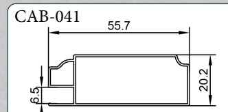
CAB-041 CABINET FRAME / GLASS
