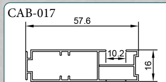
CAB-017 BACK PANEL BOARD
