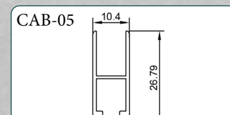
CAB-05 BOTTOM RAIL
