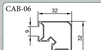
CAB-06 CORNER CONNECTOR B
