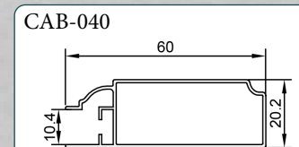
CAB-040 CABINET FRAME / BOARD
