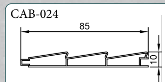
CAB-024 YP LOUVER
