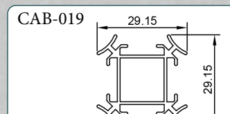
CAB-019 PANEL DIVIDER
