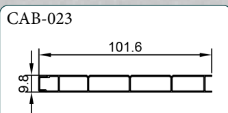
CAB-023 YP MAIN BOARD
