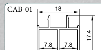
CAB-01 UPPER CAHA
