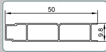
CAB-022
