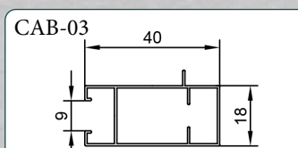
CAB-03 TOP RAIL
