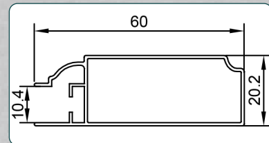
CAB-040
