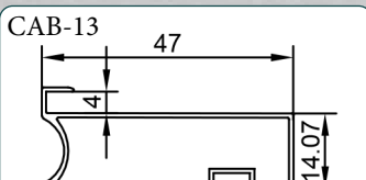
CAB-13 ACP SIDE FRAME
