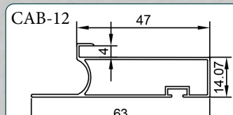
CAB-12 ACP TOP FRAME
