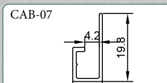
CAB-07 COVER
